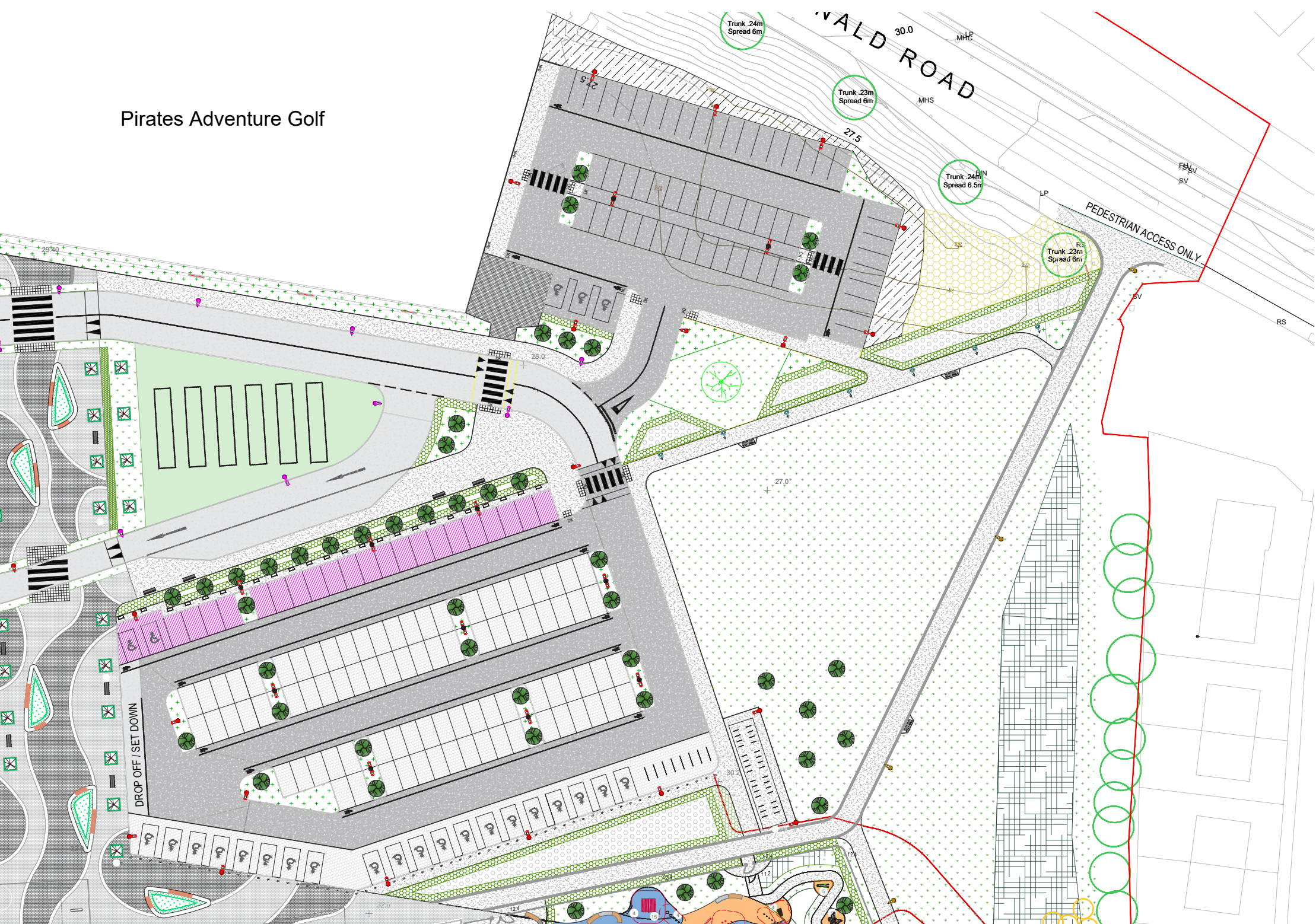
Fig 1.2 Propose Revised Design at PAG Car Park
